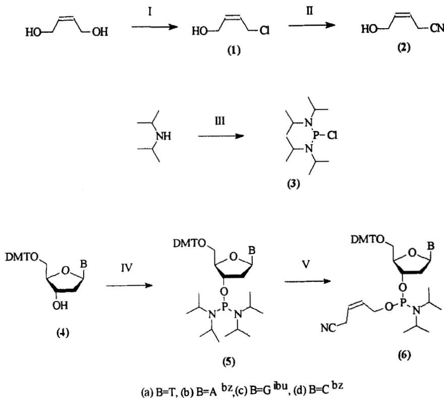
FIG. 1: I) \text{SOCl}_2 , Pyr, \text{Et}_2\text{O} , 0^\circ\text{C} ; II) KCN, NaI, MeCN, 20^\circ\text{C} ; III) \text{PCl}_3 , DCM, -60^\circ\text{C} ; IV) DIPA, (3), DCM, 20^\circ\text{C} ; V) Tetrazole, (2), DCM, 20^\circ\text{C}
